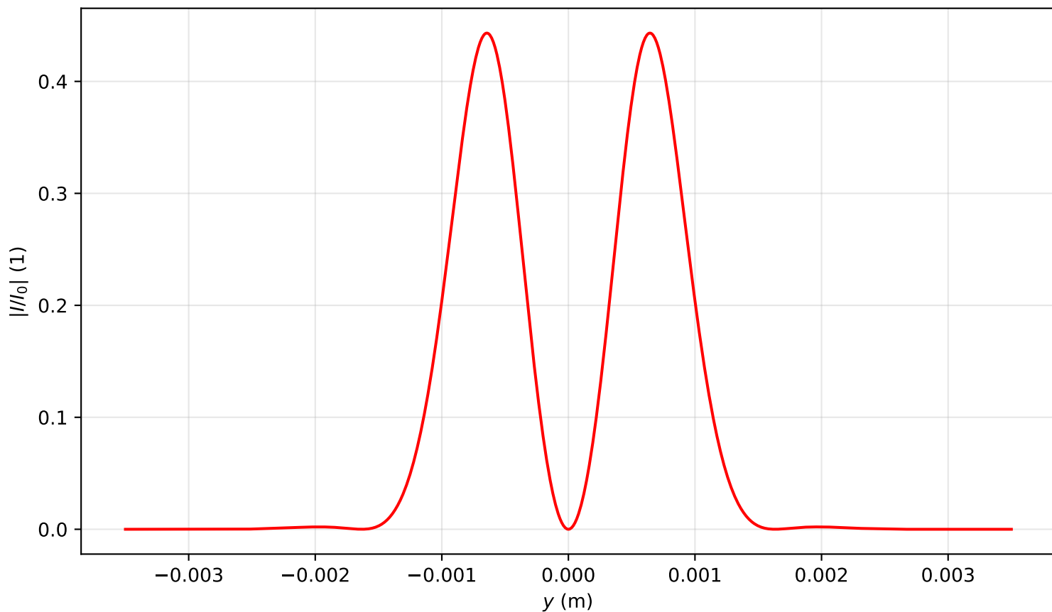
Intensity profile I(x=0, y, z=1.831)/I_0 , P_{in}=3.0P_{cr} , artificial time
